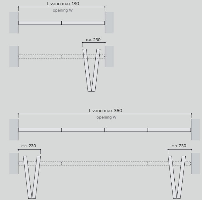
Vista in pianta Plan view
