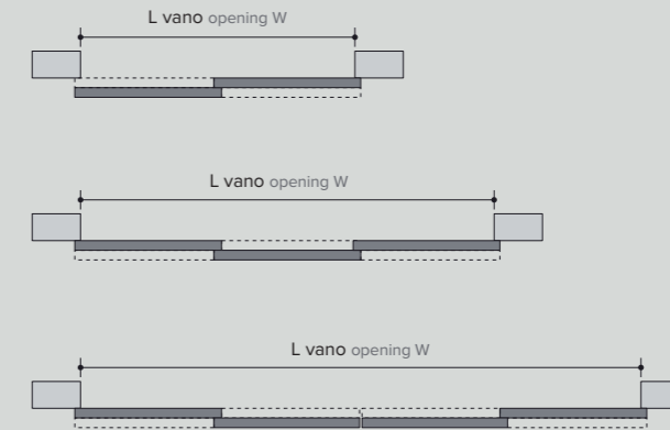
Vista in pianta Plan view
